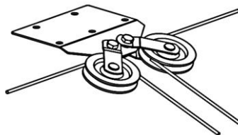
Pulley Anchor - Ceiling or Wall
